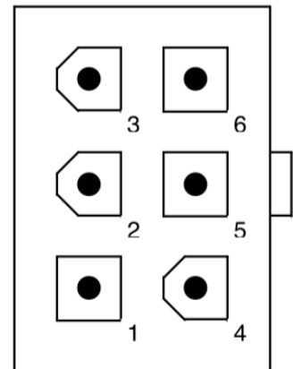
VMC / Bus Connector Face View Header (Pins)
