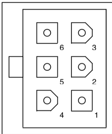
Peripheral Connector Face View Receptacle (Sockets)
